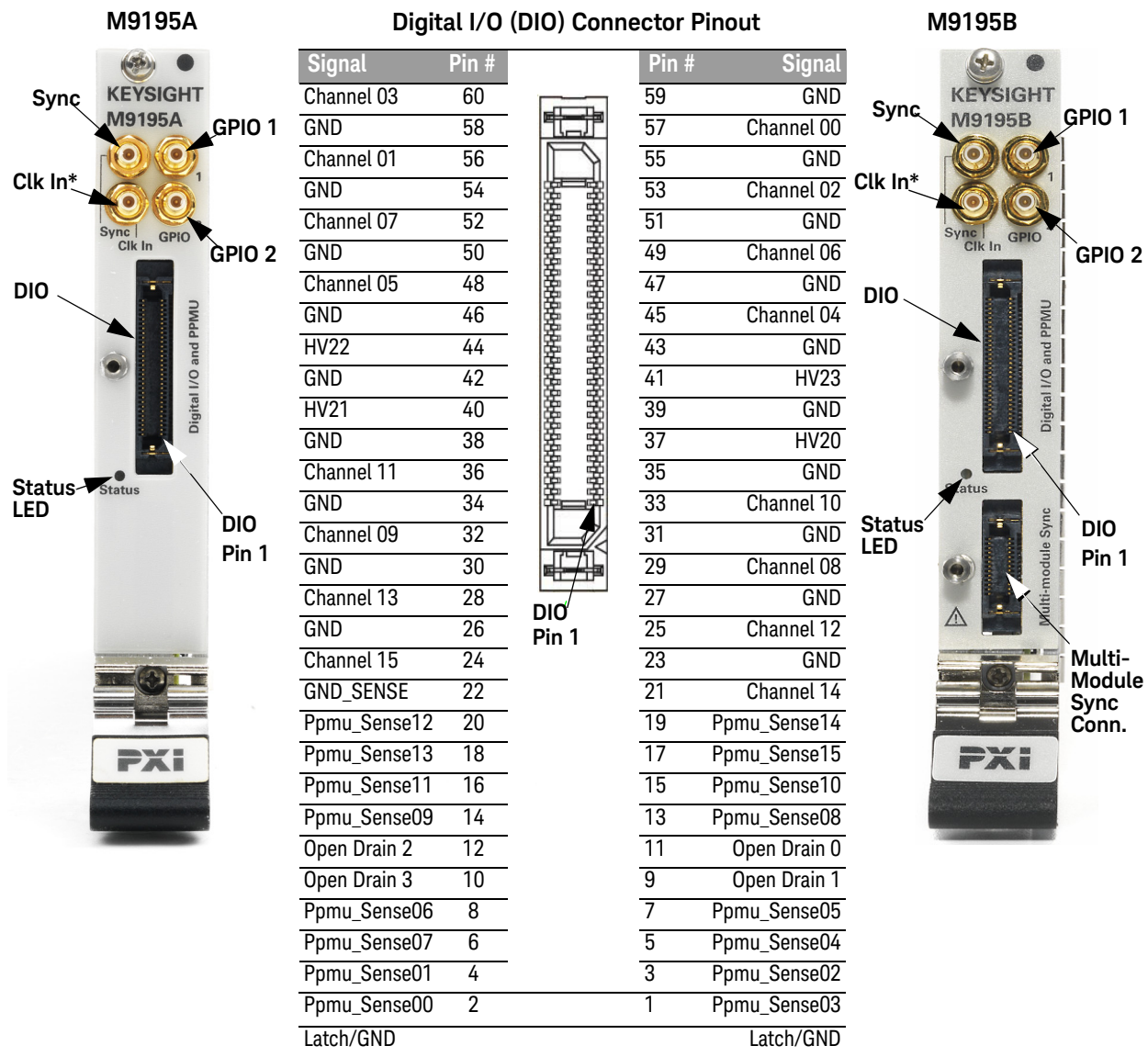
Figure 17 M9195A Front Panel and Connector Pin-out
